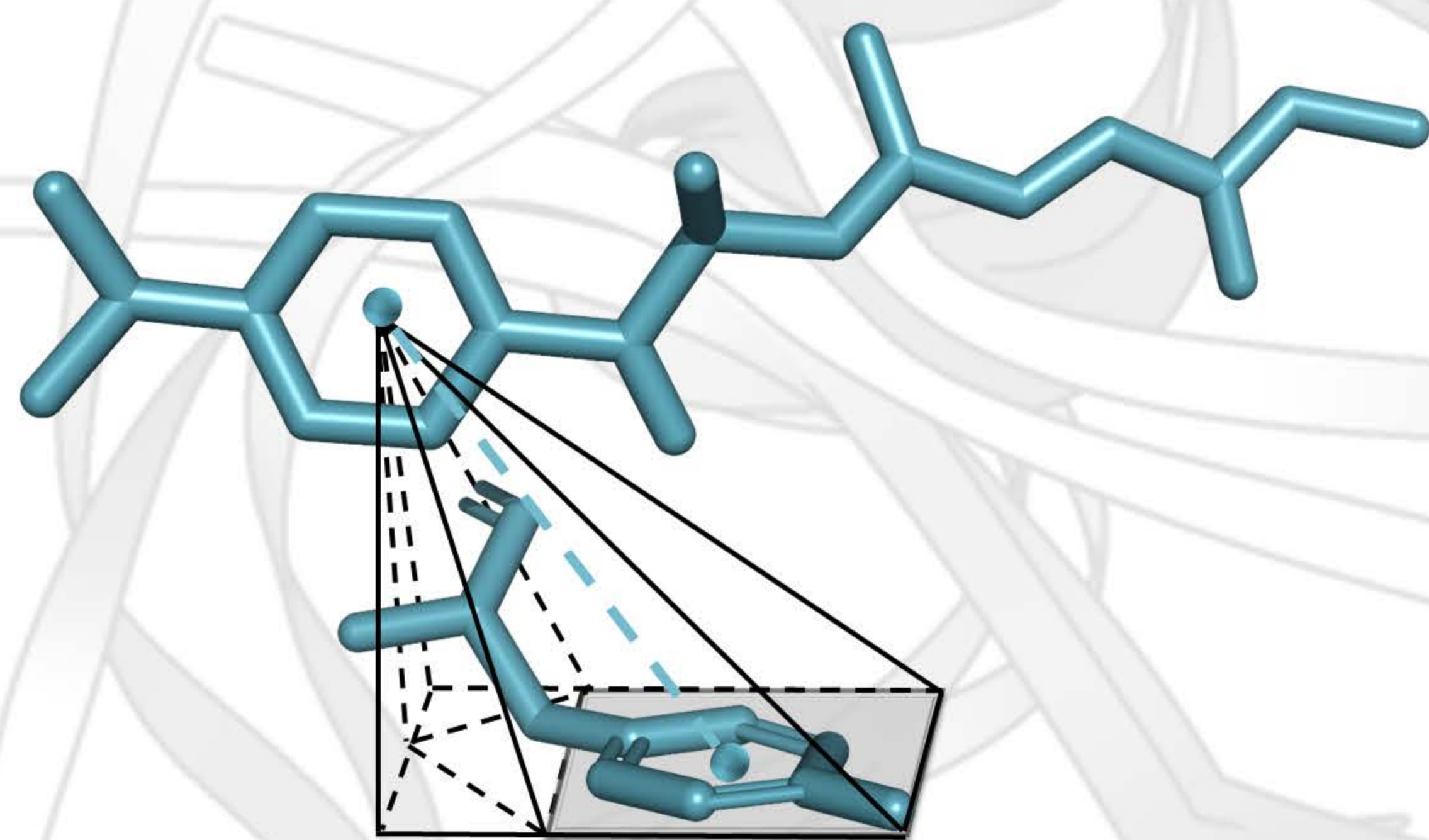
Y197 (HDAC1)
